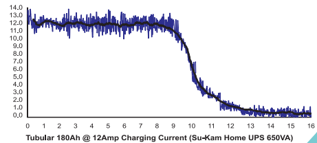
Charging Current (Ampere) Vs Time (Hrs)
