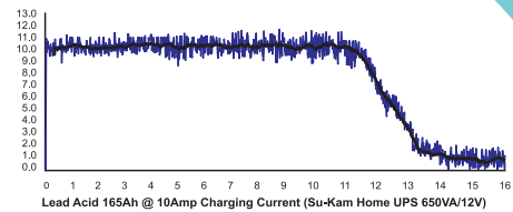
Charging Current (Ampere) Vs Time (Hrs)
